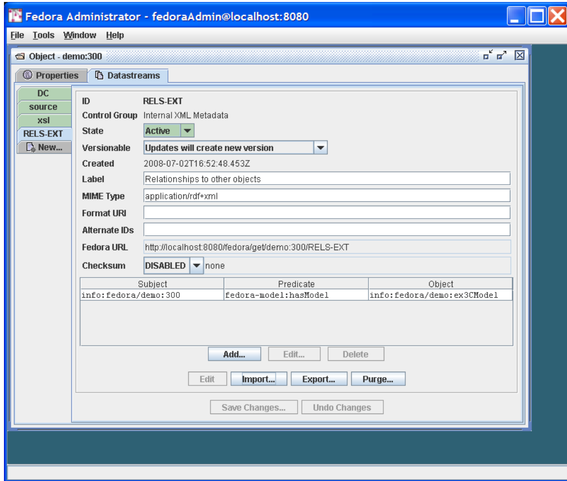
Figure 15 – Example 3 Linking a Digital Object to a Content Model
