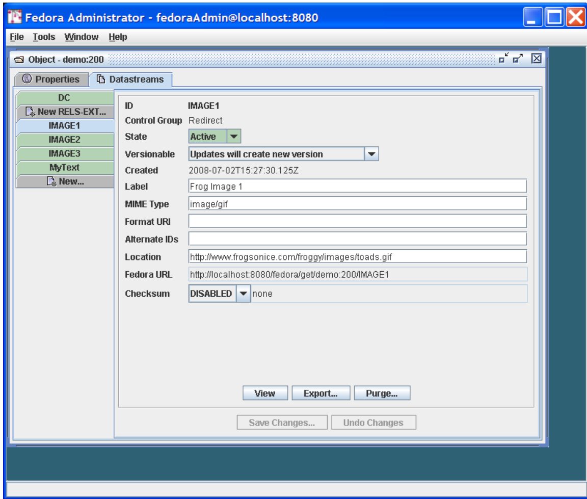
Figure 10 - Example 2 datastream display
