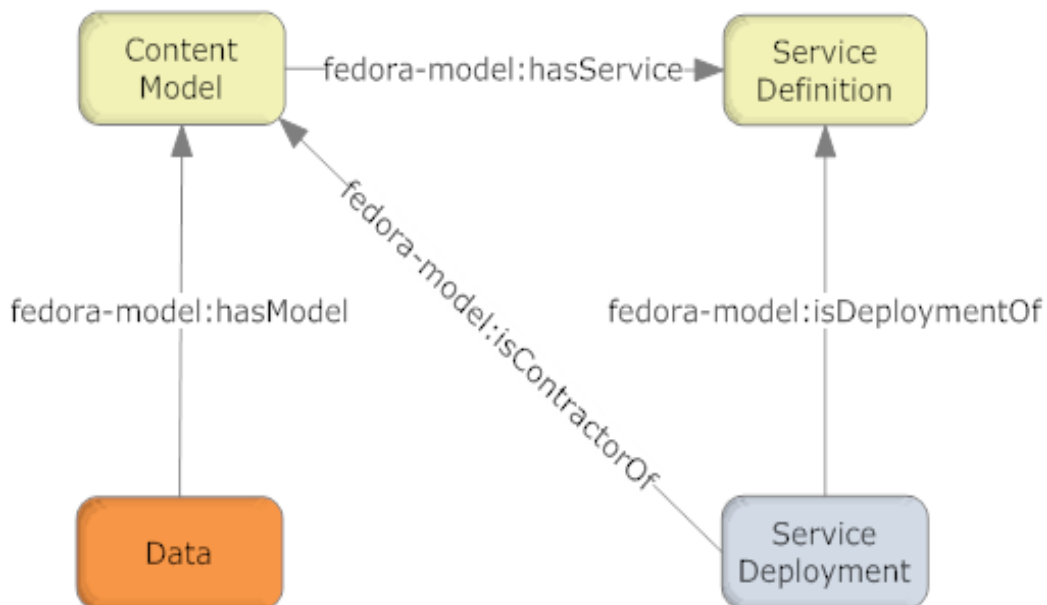
Figure 13 – Fundamental CMA Relationships
