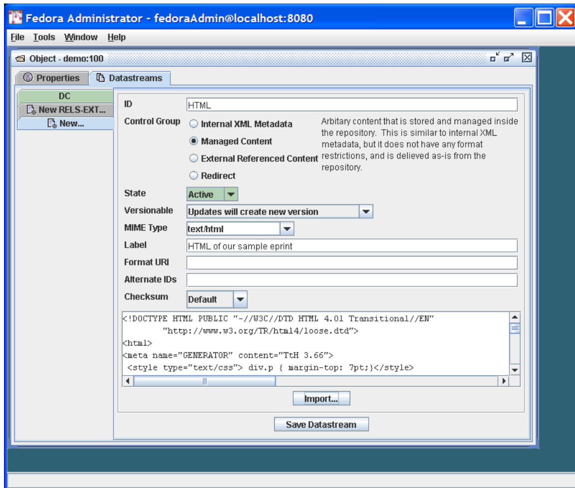
Figure 6 - Adding a new managed content datastream
